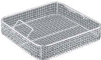
MESH TRAY SI-3536 240x250x50mm SI-3537 240x250x60mm SI-3538 240x250x70mm SI-3539 280x250x50mm SI-3540 280x250x60mm
