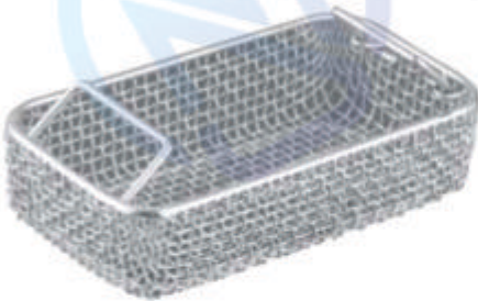
MESH TRAY SI-3522 240x130x50mm SI-3523 240x130x60mm SI-3524 240x250x50mm SI-3525 240x250x60mm SI-3526 480x250x50mm SI-3527 480x250x60mm SI-3528 480x250x70mm
